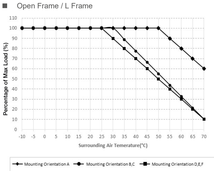
Fig.1.1 De-rating for Mounting Orientation A > 50°C de-rate power by 2% / °C De-rating for Mounting Orientation B, C > 30°C de-rate power by 2.25% / °C De-rating for Mounting Orientation D, E, F > 25°C de-rate power by 2% / °C
